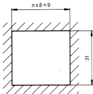
Panel cut-out
